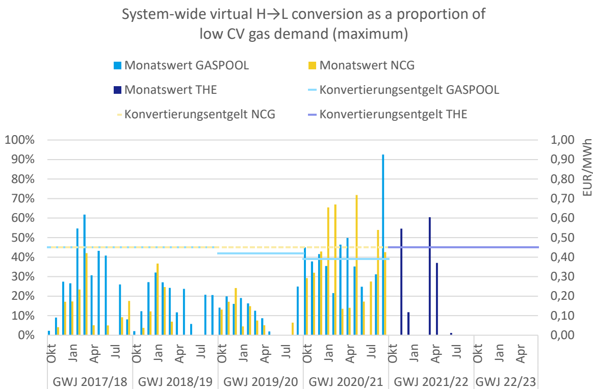
Figure 2: System-wide virtual conversion quantities as a proportion of low CV gas demand
